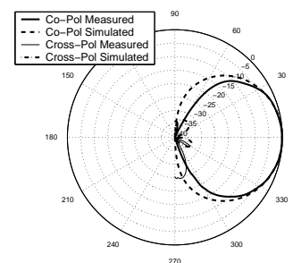
Fig. 6. E-plane Radiation Pattern - 14 GHz Array
