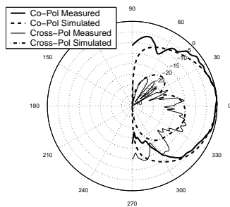
Fig. 8. E-plane Radiation Pattern - 35 GHz Array
