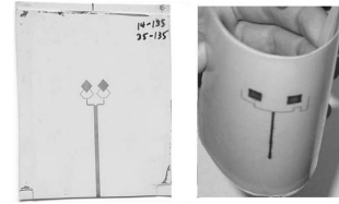
Fig. 3. Photo of the fabricated symmetrically-fed Array & Photo demonstrating flexibility
