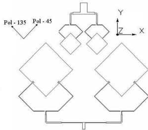
Fig. 2. Top View - Symmetrically-fed Array
