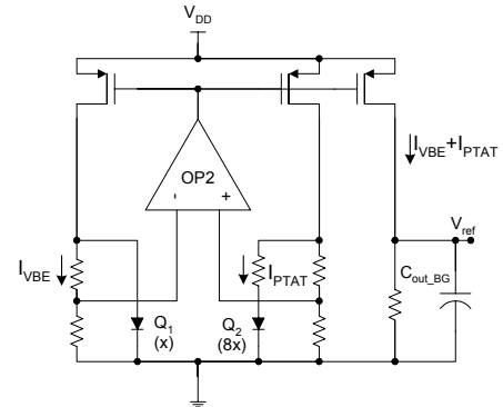
Fig. 6. Schematic of bandgap reference circuit.
