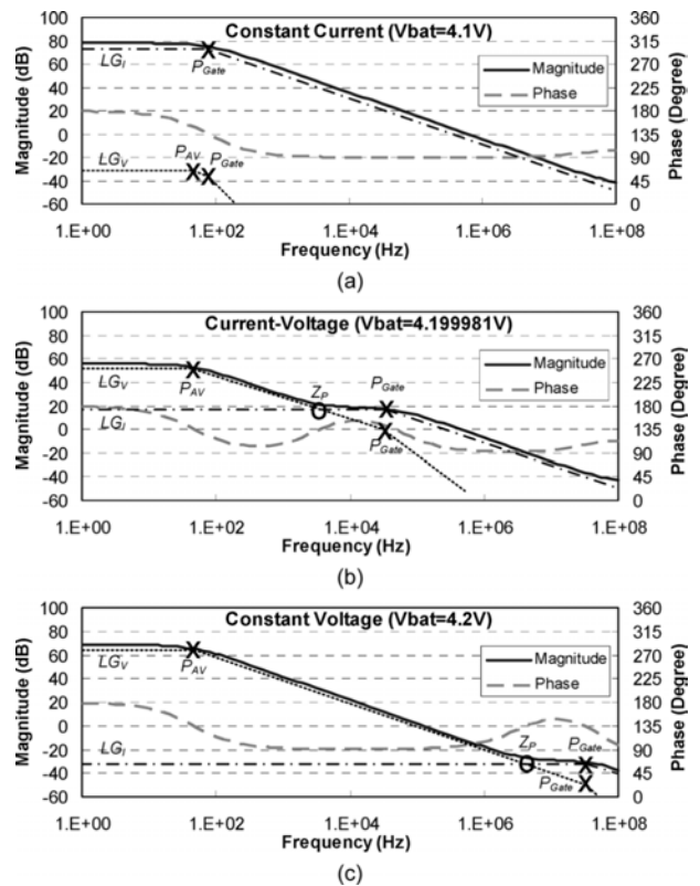
Fig. 3. Simulated bode plots during (a) CC, (b) CC-CV, and (c) CV.
