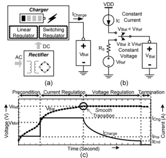
Fig. 1. (a) Typical Li-Ion battery charger and CC-CV charging (b) scheme and (c) sequence.
