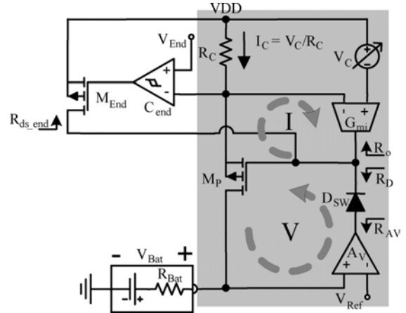
Fig. 2. Proposed charger circuit.
