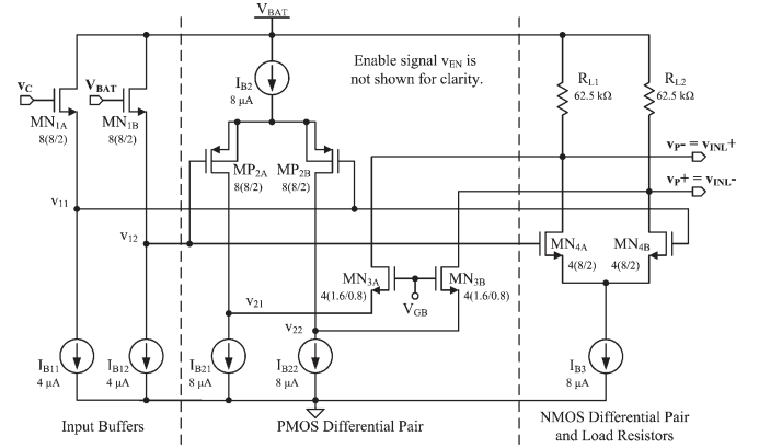
Fig. 6. Comparator CP_{REF} 's preamplifier AMP_{PRE} (all dimensions are in \mu\text{m} ).
