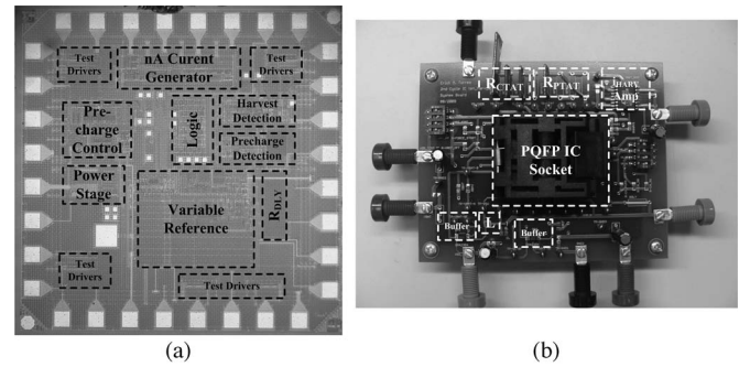
Fig. 7. (a) Die photograph of the 1.5 \times 1.5 \text{ mm}^2 energy harvester IC and (b) the PCB used to experimentally test it.
