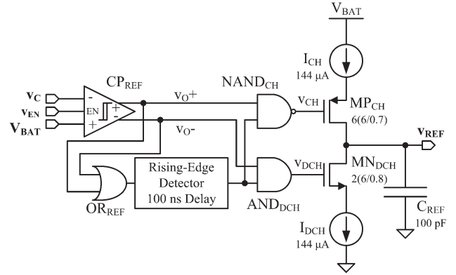
Fig. 3. Tuning reference circuit (all dimensions are in \mu\text{m} ).
