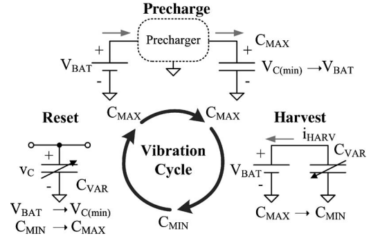
Fig. 1. Energy-harvesting phases: precharge, harvest, and reset [13].
