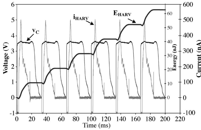
Fig. 8. Experimental measurements showing variable capacitor voltage v_C , harvesting current i_{HARV} , and extrapolated energy gain E_{HARV} .
