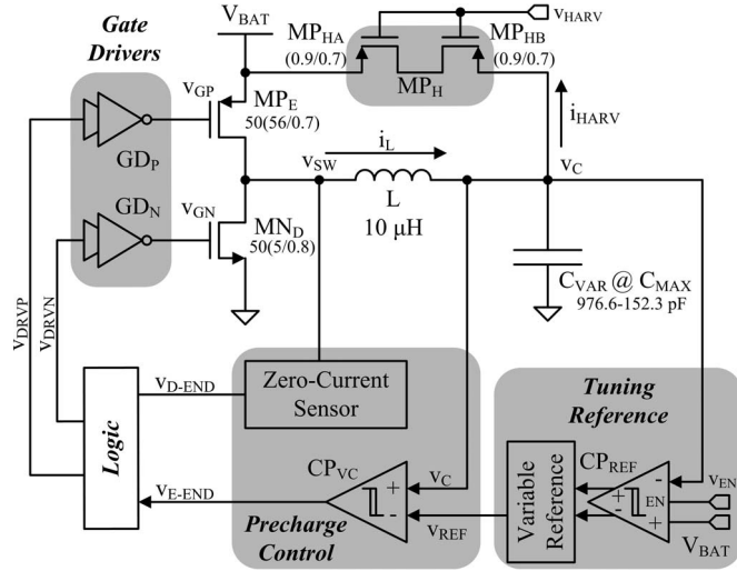
Fig. 2. Self-tuning precharger circuit (all dimensions are in \mu\text{m} ).
