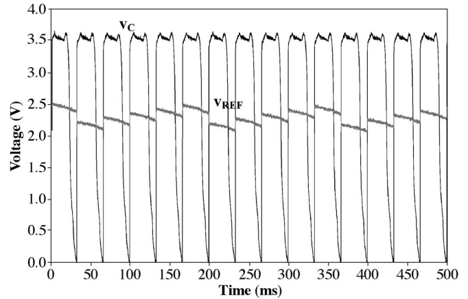
Fig. 9. Experimental waveforms showing variable capacitor voltage v_C and variable reference voltage v_{REF} .
