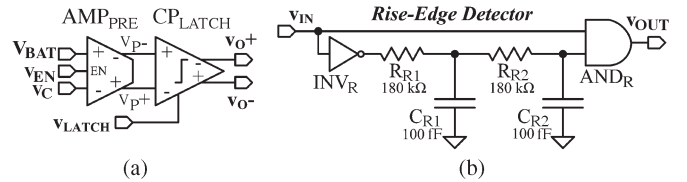
Fig. 4. (a) CP_{REF} 's preamplifier ( AMP_{PRE} ) and latching comparator ( CP_{LATCH} ) stages; and (b) 100-ns delay rising-edge detection circuit.
