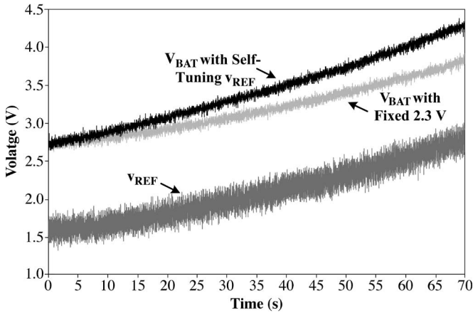
Fig. 11. Experimental voltage profile of a 1- \mu F capacitor when charged with the energy harvester IC with the proposed self-tuning v REF and a fixed 2.3-V reference.
