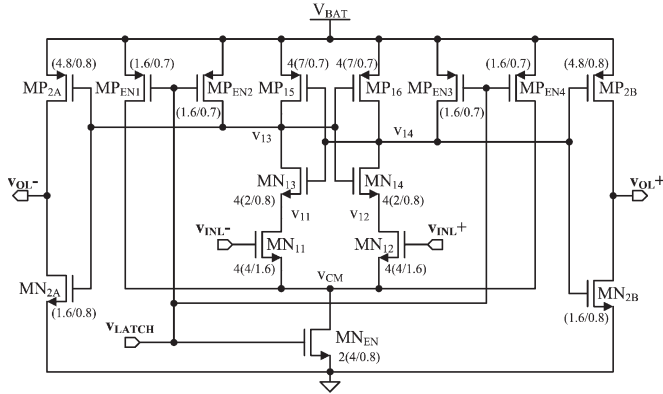
Fig. 5. Comparator CP_{REF} 's latch CP_{LATCH} (all dimensions are in \mu\text{m} ).
