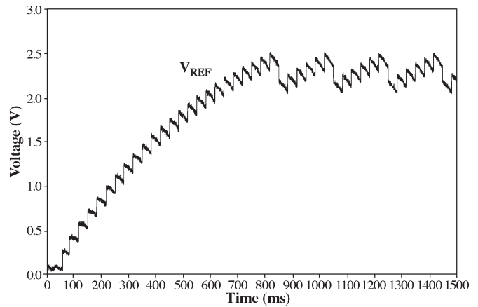
Fig. 10. Prototyped variable v_{REF} during startup and through steady state.
