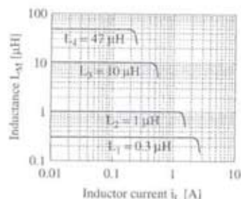
Fig. 2. Typical inductance-saturation graph [17]
