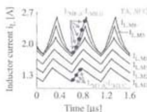
Fig. 4. Experimental inductor-current waveforms as a 1- \mu H inductor saturates
