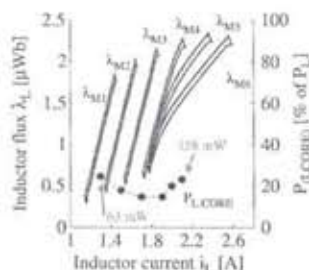
Fig. 6. Flux-current loops and resulting impact of core losses
