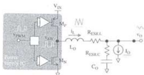
Fig. 3. Switching buck DC-DC converter
