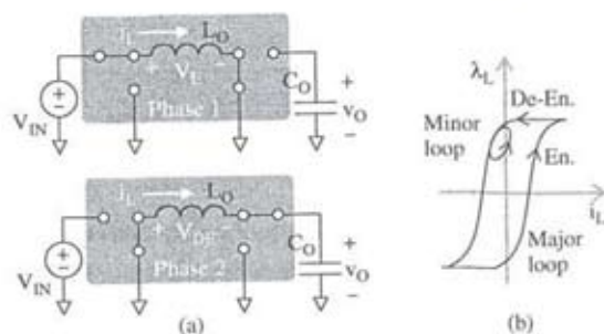
Fig. 1. (a) Energizing and de-energizing inductor L_O (b) means flux increases and decreases along L_O 's hysteresis loop
