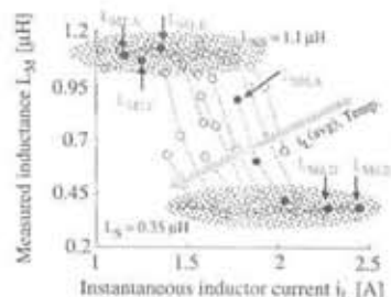
Fig. 5. Measured (and overlapped) inductances across current and temperature (at 30, 60, and 90 °C)
