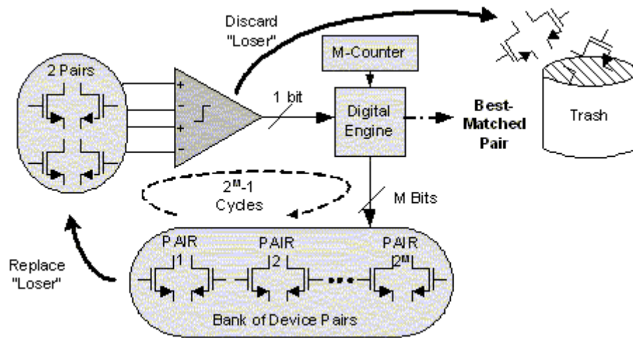
Figure 2. Survivor strategy
