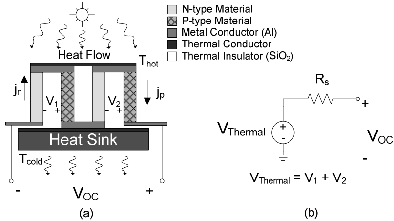
Figure 4. (a) Thermoelectric energy converter composed of two series thermocouples and (b) its circuit model.
