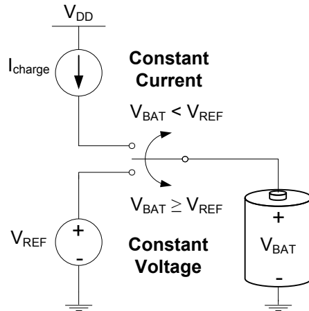
Figure 7. Constant-current/constant-voltage model.
