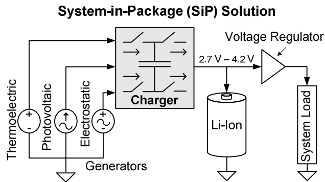
Figure 9. Electrical diagram of the proposed system-in-package (SiP) micro-sensor.
