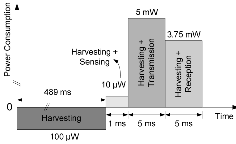
Figure 10. Power profile of the system in a 500 ms cycle.
