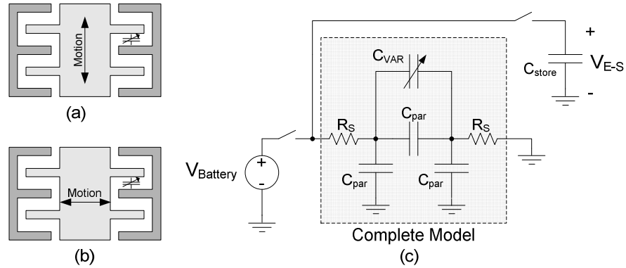
Figure 3. (a) Gap and (b) overlap in-plane variable capacitors, and (c) an energy harvesting circuit highlighting the model of the variable capacitor.
