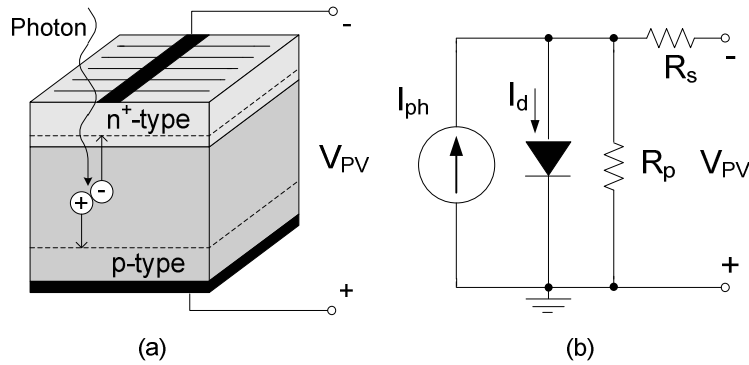
Figure 5. (a) Photovoltaic cell and (b) its circuit model.
