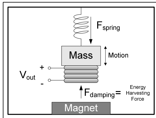
Figure 1. Electromagnetic vibration energy harvester.
