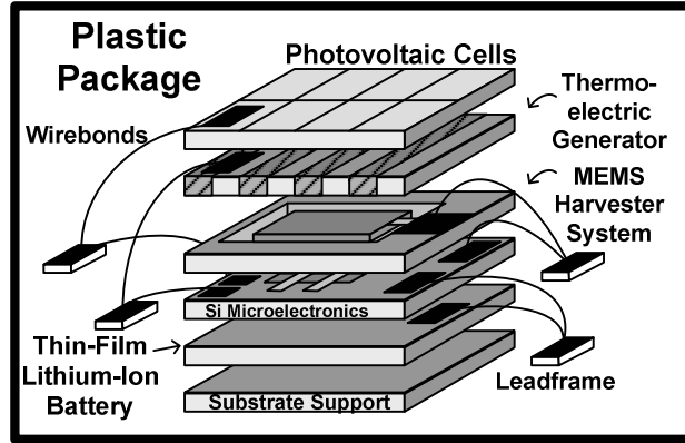
Figure 8. Physical profile view of the proposed system-in-package (SiP) micro-sensor.
