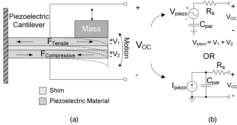
Figure 2. (a) Piezoelectric “bimorph” beam and its (b) Thevenin and Norton equivalent circuit models.
