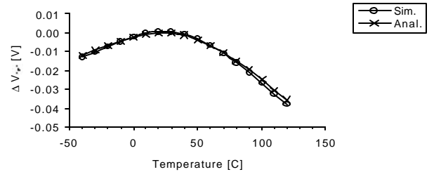
Figure 5. Comparison of simulated and analytical \Delta V_{ref} for resistor TCs of 5 \times 10^{-4}/^\circ\text{C} and 2 \times 10^{-4}/^\circ\text{C}^2 .
