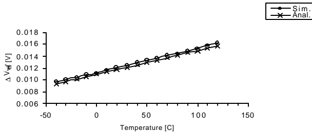
Figure 3. Comparison of simulated and analytical \Delta V_{ref} for a resistor mismatch of 2%.
