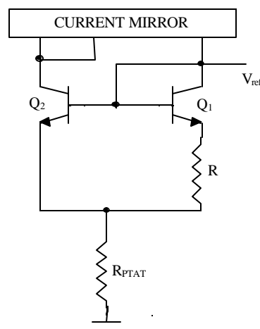
Figure 1. Basic cell.
