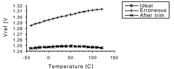
Figure 11. Ideal and erroneous reference voltage (before and after trimming) for the case of current-mirror mismatch.
