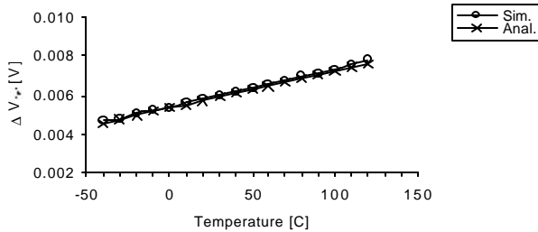
Figure 6. Comparison of simulated and analytical \Delta V_{\text{ref}} for a transistor mismatch of 2%.
