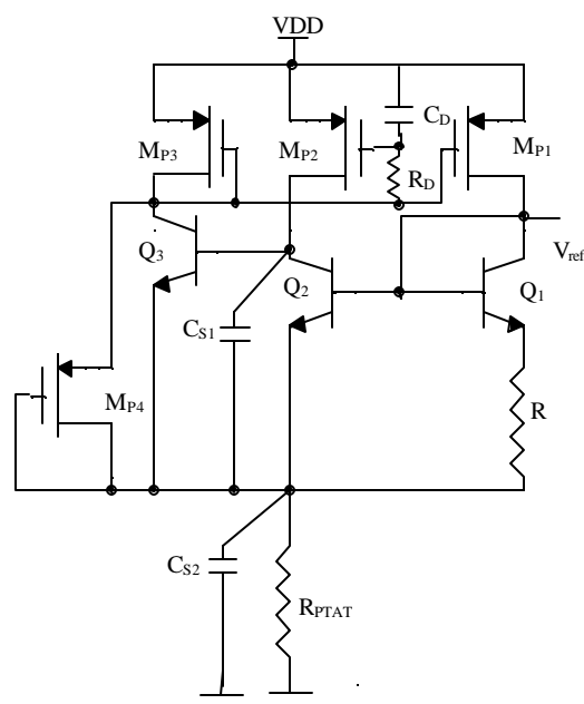
Figure 2. A first-order bandgap reference.
