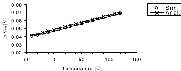
Figure 7. Comparison of simulated and analytical \Delta V_{\text{ref}} for a current-mirror mismatch of 10%.
