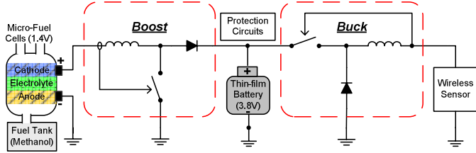
Fig. 5. Hybrid FC-Li-Ion energy- and power-conditioning system.
