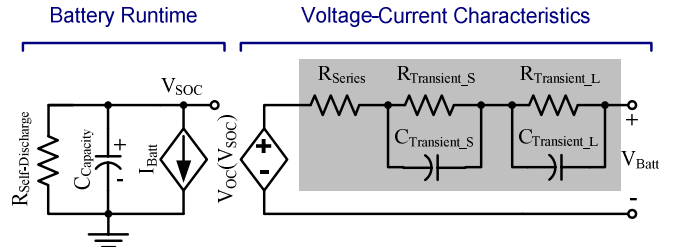
Fig. 7. Thin-film Li-Ion model.
