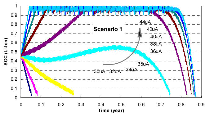
Fig. 8. Lifetime: Li-Ion's state-of-charge (SOC) for various I_{FC} 's.
