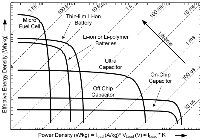
Fig. 3. Ragone plot: energy and power densities of various devices [15-16].
