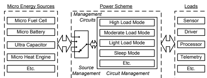
Fig. 1. Micro-scale electronic system diagram.
