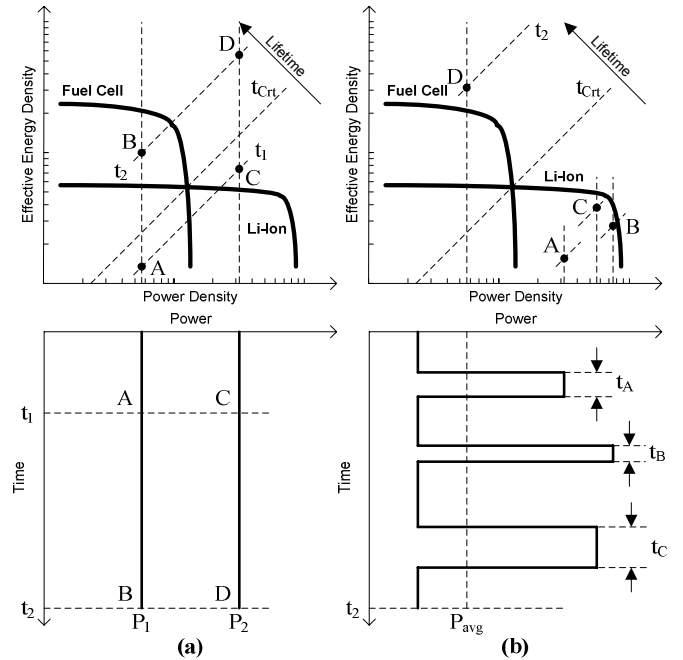
Fig. 4. Energy source mappings for (a) constant and (b) time-dependent loads.
