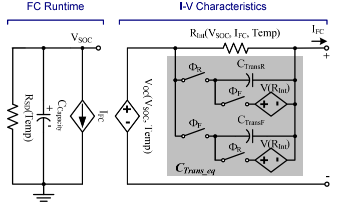
Fig. 6. Micro-scale FC model.
