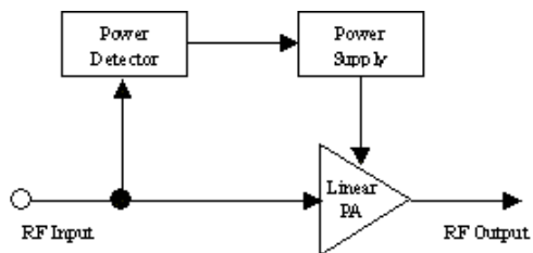
Figure 4. Power tracking supply
