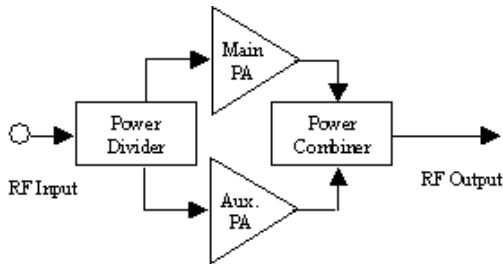
Figure 2. Dual PA power-sharing approach
