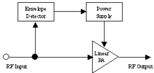
Figure 3. Envelope-following supply scheme
