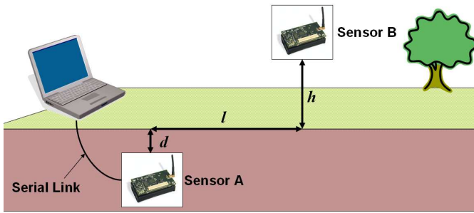
Fig. 1. Experimental setup.
