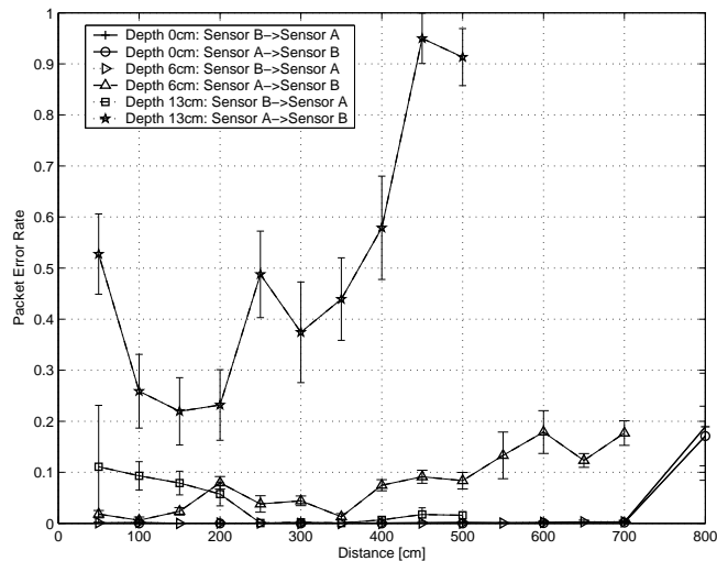
Fig. 5. Packet error rate for elevated remote sensor.
