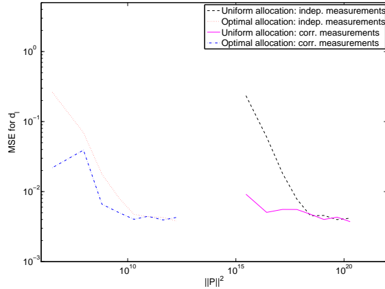
Figure 4: The rate-distortion curves calculated through simulated measurements. Measurements were simulated directly through independent random generation. Correlated measurements were also simulated by generating random environmental fields from a piecewise linear class and taking the resulting sensor measurements.
