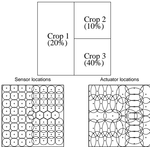
Figure 2: An example WSN for a stylized agricultural irrigation application. A field 100m on each edge has three crops with varying desired soil moisture percentages. A collection of moisture sensors (bottom left) and irrigation actuators (bottom right) are deployed, with a single contour denoting where the influence field has mostly vanished.
