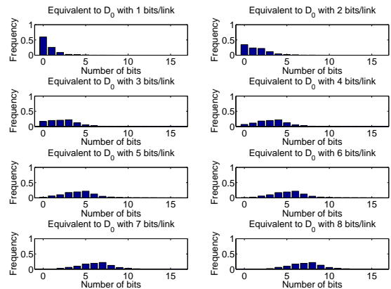
Figure 3: The rate-distortion curve comparing MSE estimation error for a single actuation coefficient d_l and the total network power needed to achieve that distortion are shown in the top plot. The bit allocations resulting from the optimal power scheduling algorithm achieve the same distortion using significantly less total power than a uniform bit allocation strategy. The bottom plot indicates the distribution of bits on each communication link. Each pane corresponds to the distortion equivalent of a uniform bit allocation scheme. The bars indicate the fraction of links using that number of bits.
