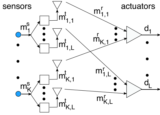
Figure 1: A schematic of the communications pathways in the WSAN model. The k^{\text{th}} sensor makes a noisy reading m_k^s . The quantized measurement m_{k,l}^t with B_{k,l} bits of precision is sent to the actuator l^{\text{th}} actuator. After incurring bit errors in the wireless channel, the measurements m_{k,l}^r are received by the actuator and used to form the approximate actuation coefficient \hat{d}_l .
