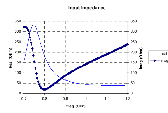
Figure 3. Input impedance of the simulated RFID antenna
