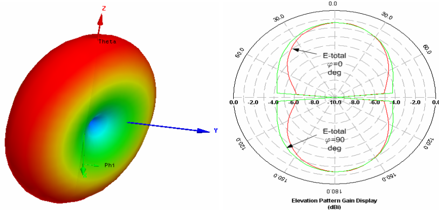
Figure 4. 3-D and 2-D far-field radiation plots.
