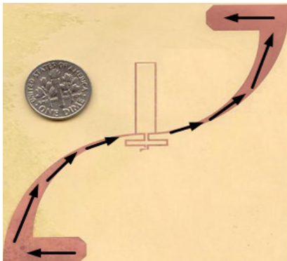
Figure 2. Fabricated RFID antenna and single dipole antenna direction of current flow
