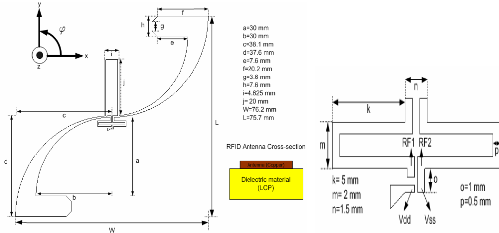
Figure 1. RFID Antenna structure and double inductive stub matching network
