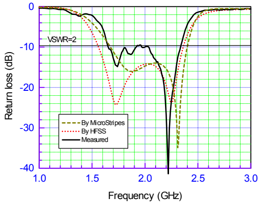
Fig. 3. Measured and simulated results for return loss of the low profile broadband two-strip monopole antenna.
