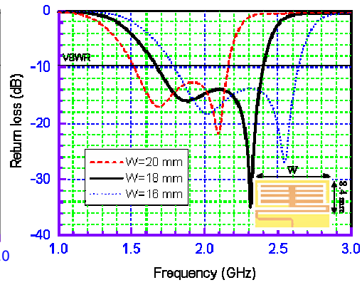
Fig. 4. Effect of the width ( W ) on the operating frequency of a two-strip monopole antenna.
