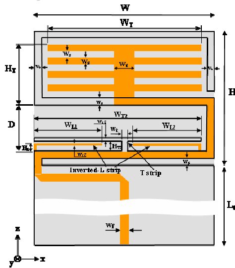
Fig. 5. Configuration of a broadband and dual-frequency two-strip monopole antenna. [Geometrical parameters: H=12 mm ( 0.08\lambda_0 ), W=16 mm ( \sim 0.11\lambda_0 ), H_T=10.8 mm, W_T=13.9 mm, D=4.2 mm, W_T=1.8 mm, H_T=1.0 mm, W_T=14.8 mm, H_L=0.75 mm, W_{L1}=W_{L2}=6.0 mm, w_s=0.6 mm, w_{s2}=0.25 mm, w_f=0.5 mm, w_f=0.76 mm, t=0.254 mm, and L_g=20 mm.]
