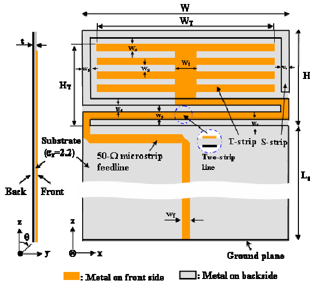
Fig. 1. Geometry of a broadband two-strip planar monopole antenna, which includes an S-strip on the front side and a T-strip on the backside of a planar substrate. [Geometrical parameters: H=8.4 mm ( 0.056\lambda_0 ), W=18 mm ( 0.12\lambda_0 ), H_T=7.2 mm, W_T=15.6 mm, W_t=1.8 mm, w_f=0.76 mm, t=0.254 mm, and L_g=20 mm.]
