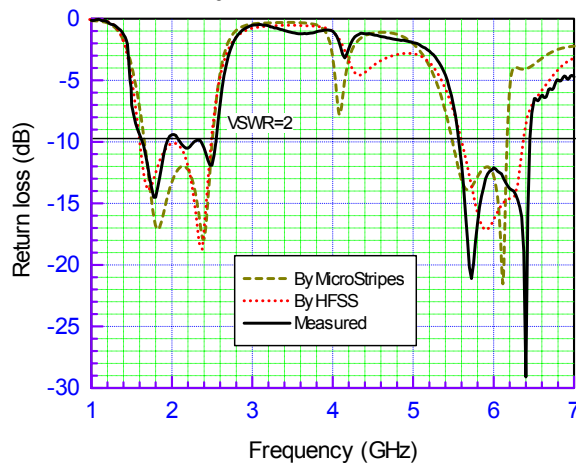
Fig. 7. Measured and simulated results for return loss of the dual-frequency two-strip antenna.
