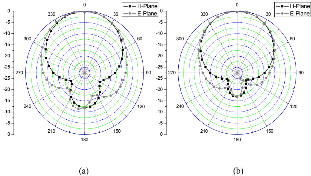
Figure 3. The radiation characteristics at 61.5 GHz of patch antennas (a) with the soft surface and (b) with the soft surface and the stacked cavity
