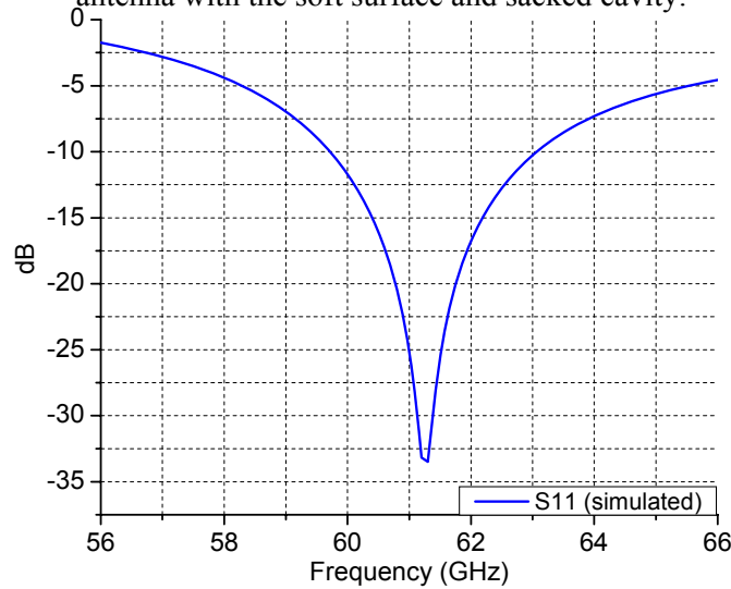
Figure 2. The simulated return loss (S11) of a patch antenna with the soft surface and the stacked cavity.
