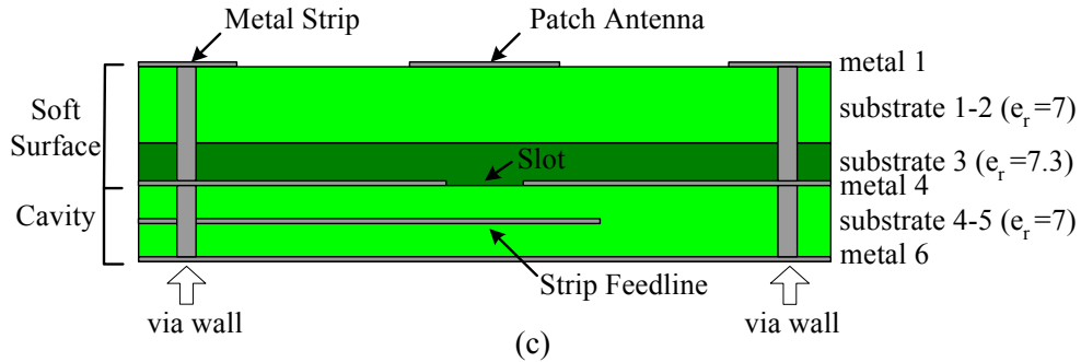
Figure 1. (a) The 3D overview (b) cross-section view (c) cross-section view of a patch antenna with the soft surface and sacked cavity.
