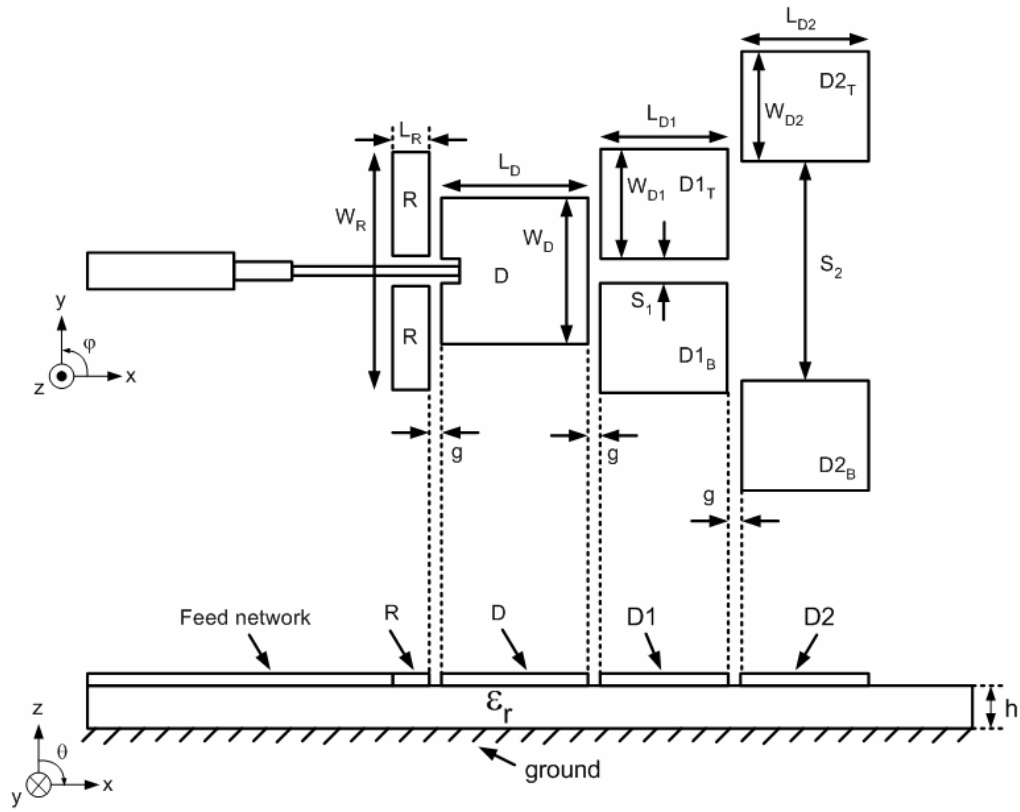
Fig. 3. Illustration of original microstrip Yagi array antenna
