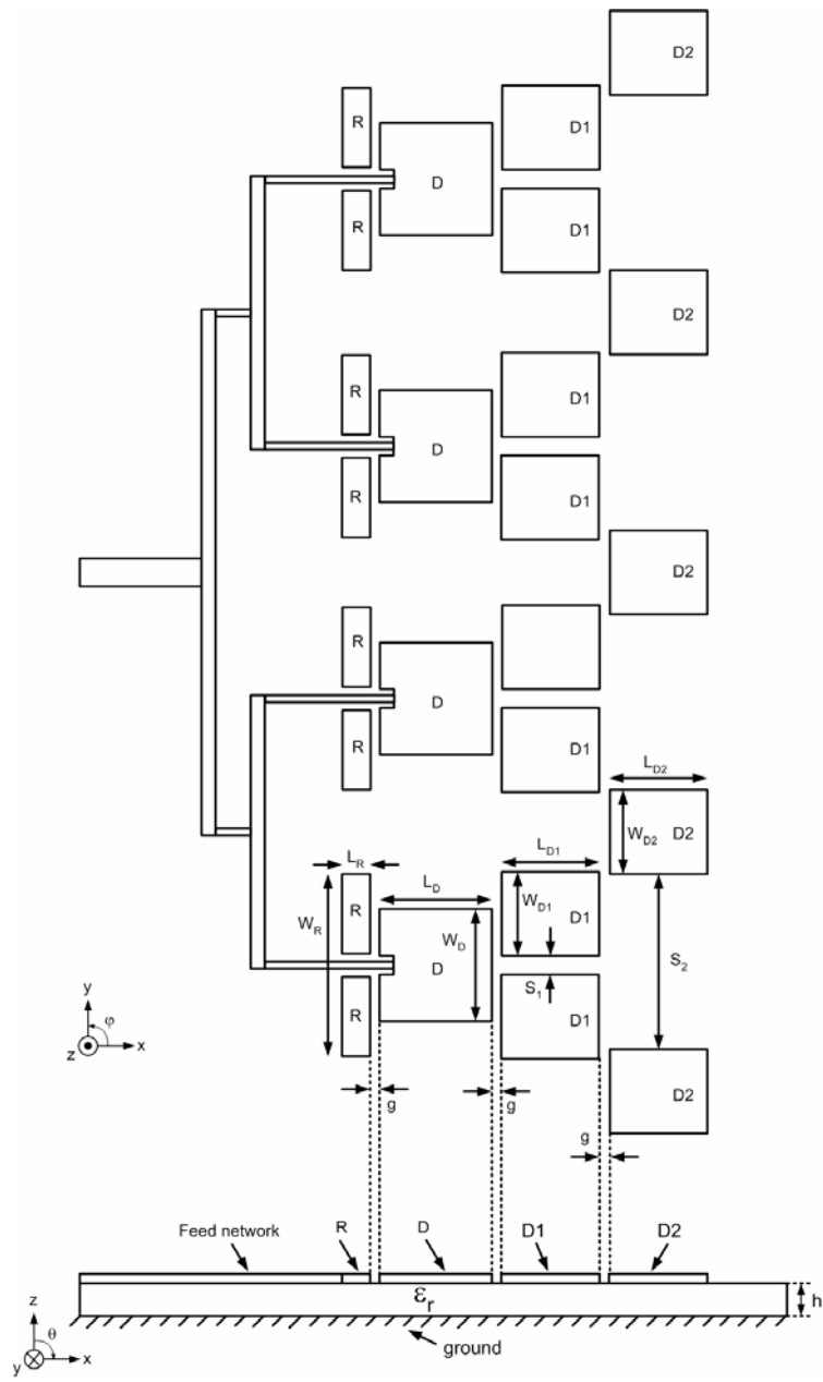
Fig. 2. Illustration of microstrip quad-Yagi array antenna
