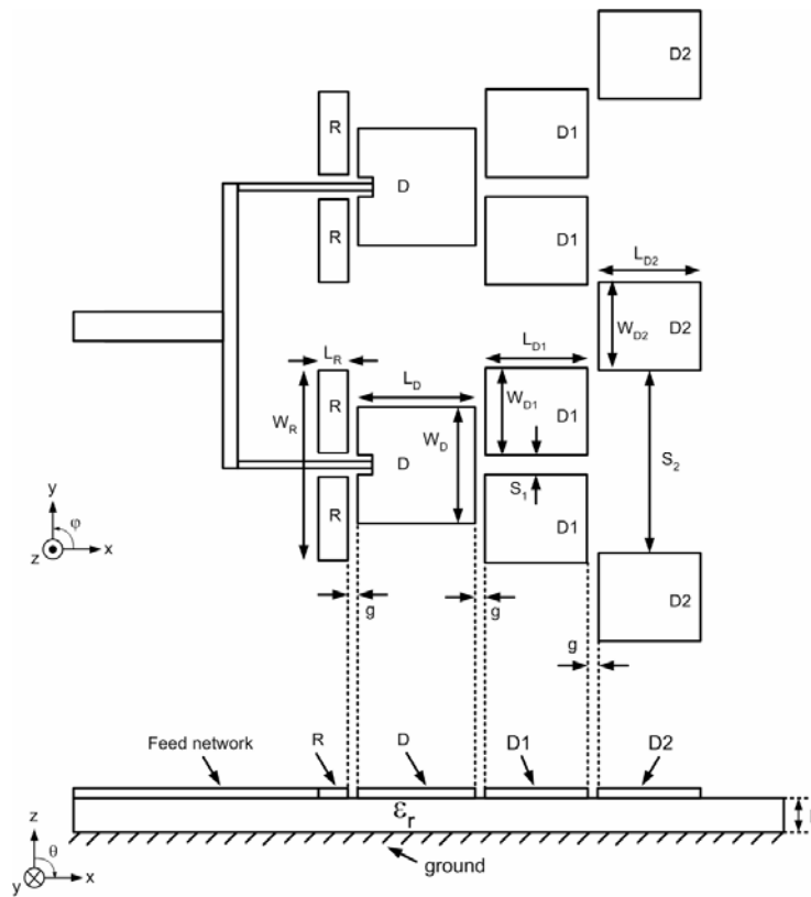
Fig. 1. Illustration of microstrip bi-Yagi array antenna
