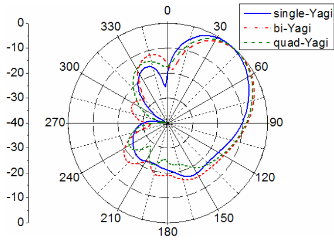
Fig. 6. Simulated 2D radiation patterns of the three Yagi arrays at 5.2 GHz.
