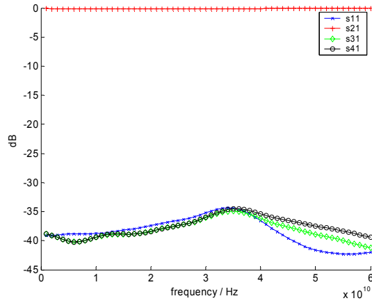
Fig.4 S-parameters for case S=42, W=12, G=252, D=0, H=10 [ \mu\text{m} ]
