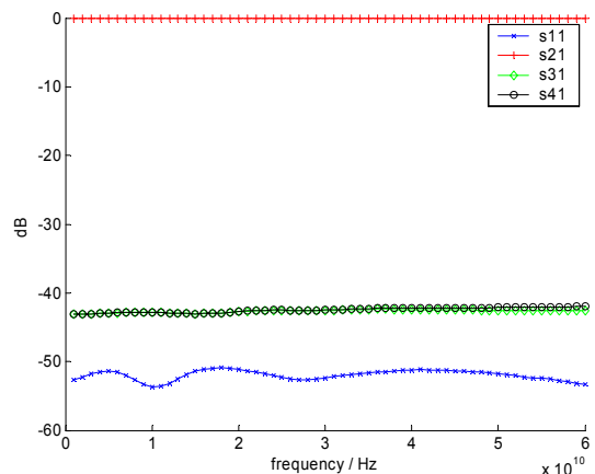
Fig.3 S-parameters for case S=42,W=12,G=84,D=24,H=10, [ \mu\text{m} ]
