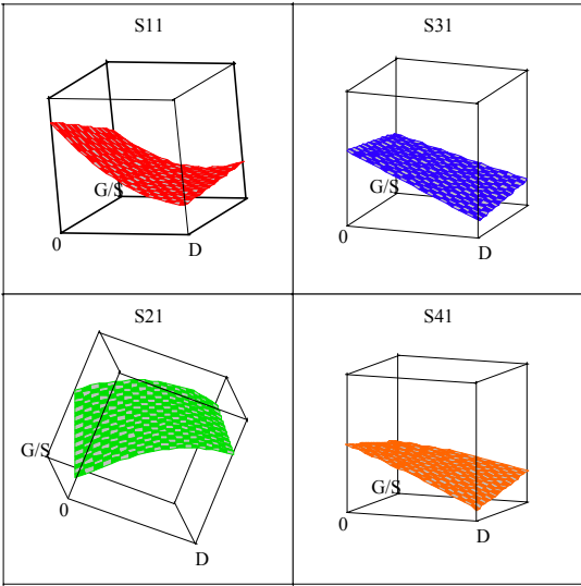
Fig.5 Surfaces representing possible solutions achieved by applying the constraint W/S=0.285
