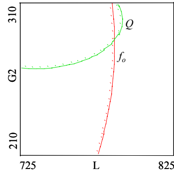
Figure 3. Surfaces of possible solutions for optimized f_0 and Q
