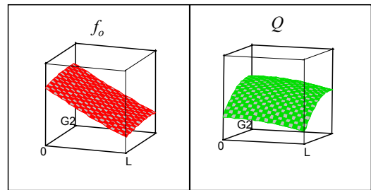
Figure 3. Surfaces of possible solutions for optimized f_0 and Q
