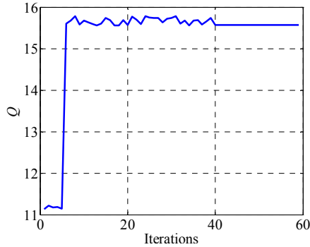
Figure 5. Convergence for two-factor GA optimization
