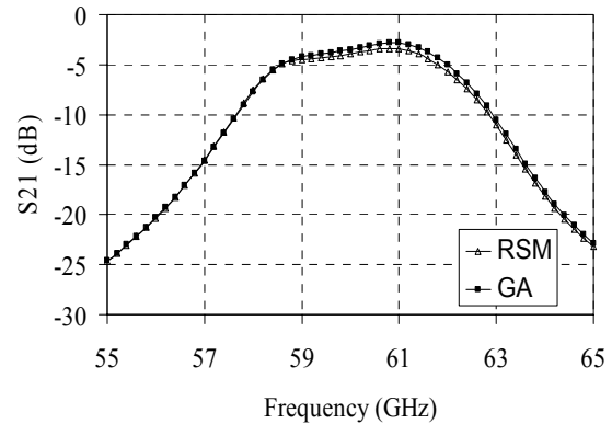
Figure 6. Comparison of the performance of the optimized filter using the two methods.
