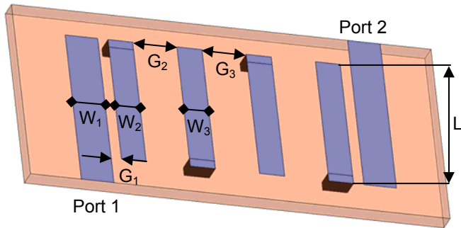
Figure 1. 3D schematic of the interdigitated passband filter.
