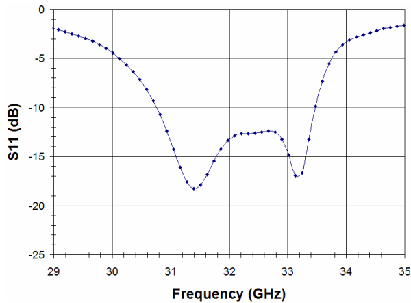
Fig. 14. Return loss versus frequency at 32.7 GHz for Fig. 13 design.
