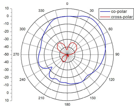
Fig. 9. E-plane co-polar and cross-polar component on elevation plane for 32.5 GHz.
