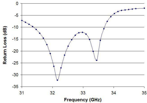
Fig. 8. Simulated return loss versus frequency for 32.5 GHz design
