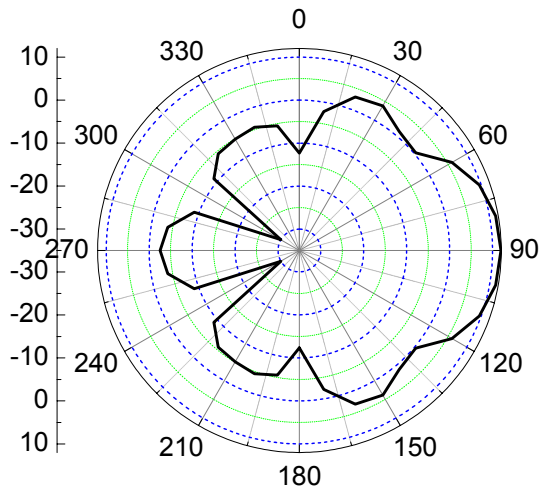
Fig. 4 Simulated 7 element Yagi radiation pattern on the vertical plane
