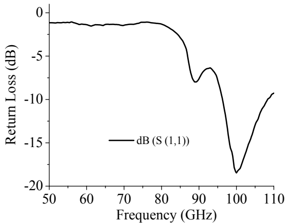
Fig. 6 Measured return loss for 5-element array
