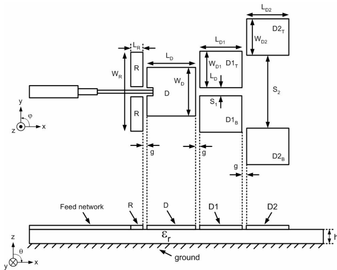
Fig. 13. Antenna structure of improved microstrip Yagi antenna
