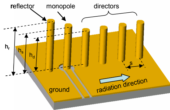
Fig. 1 The structure of W-band vertical Yagi-Uda antenna
