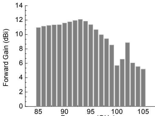
Fig. 5 Simulated forward gain vs. Frequency for 7 element array
