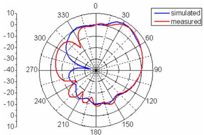
Fig. 12. Co-polarized component on elevation plane at 5.2 GHz for Fig. 7 design.
