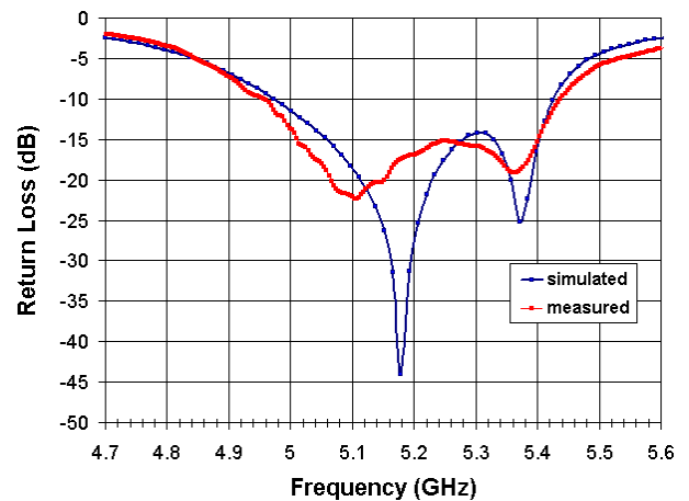
Fig. 11. Return loss versus frequency at 5.2 GHz for Fig. 7 design.
