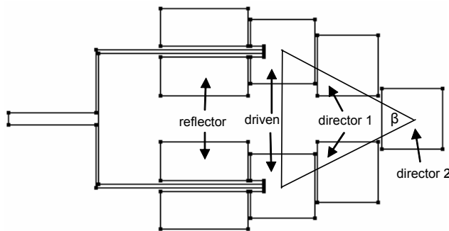
Fig. 7 Microstrip Yagi antenna structure
