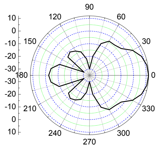
Fig. 3 Simulated 7 element Yagi radiation pattern on the horizontal plane
