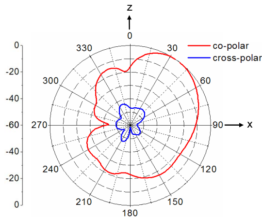
Fig. 14. E-plane co-polar and cross-polar component on elevation plane at 32.7 GHz for Fig. 12 design.
