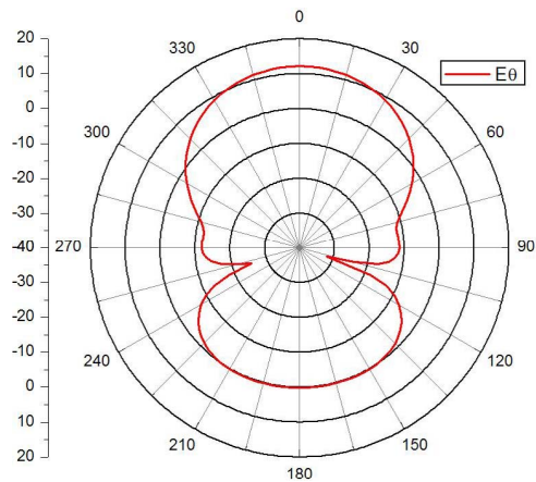
Fig. 10. E_0 component on azimuth plane for 32.5 GHz design.
