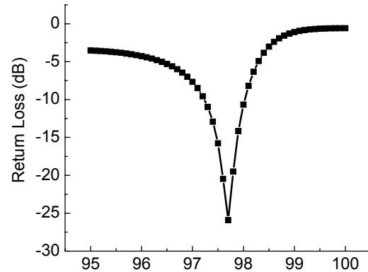
Fig. 2 Simulated return loss for 5 elements Yagi-Uda array
