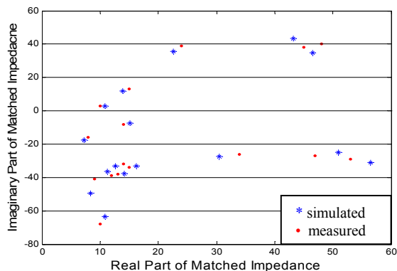
Fig. 4. Plot of measured and simulated matched impedances at 20GHz
