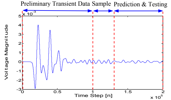
Fig. 2. The FDTD time response of 0001 impedance matching of RF MEMS tuner.
