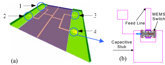
Fig. 1. (a)Diagram of simulated ‘2-bit x 2bit’ RF-MEMS tuner and (b) RF-MEMS capacitive stub
