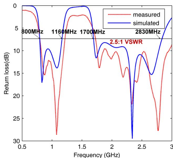
Fig. 6. Comparison between the measured and simulated results for return loss of the multiband planar antenna.
