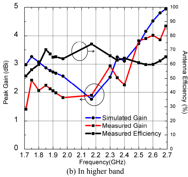
Fig. 8. Comparison between the measured and simulated results for peak gain of the multiband planar antenna and the measured antenna efficiency.
