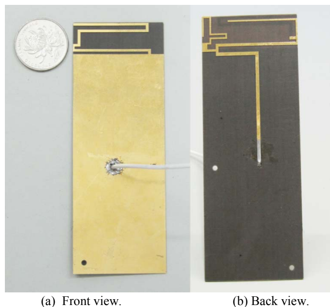
Fig. 5. Photographs of the multiband planar antenna with the optimized geometric parameters.
