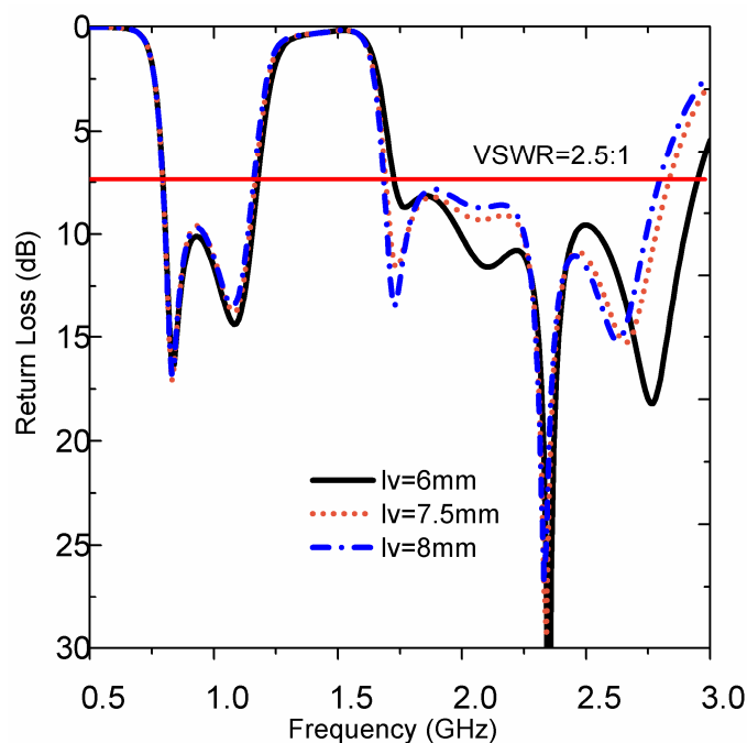
Fig. 4. Effect of the length ( l_v ) of meandered strip on the return loss of the multiband planar antenna, where l_v was changed from l_v=6 mm to l_v=8 mm. The optimized value for l_v is \sim 7.5 mm.
