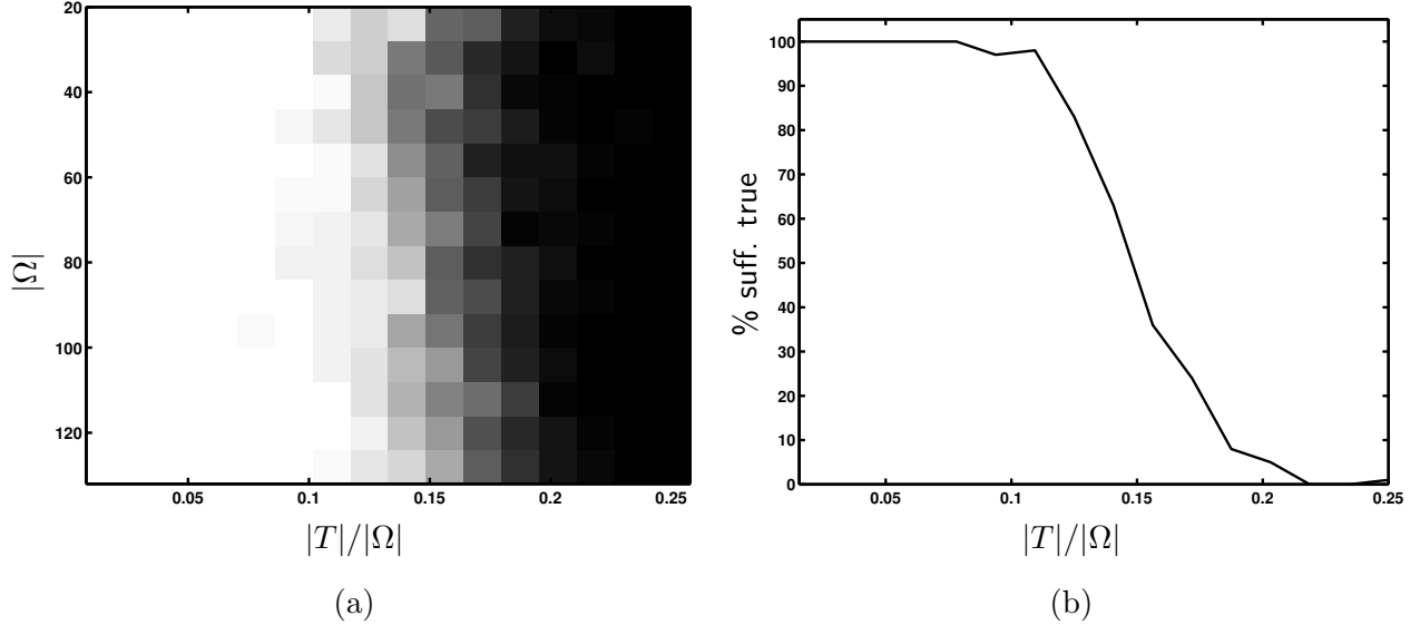
Figure 3: Sufficient condition test for N = 512 . (a) The image intensity represents the percentage of the time P(t) chosen as in (2.3) meets the condition |P(t)| < 1, t \in T^c . (b) A cross-section of the image in (a) at |\Omega| = 64 . Note that the axes are scaled differently than in Figure 2.
