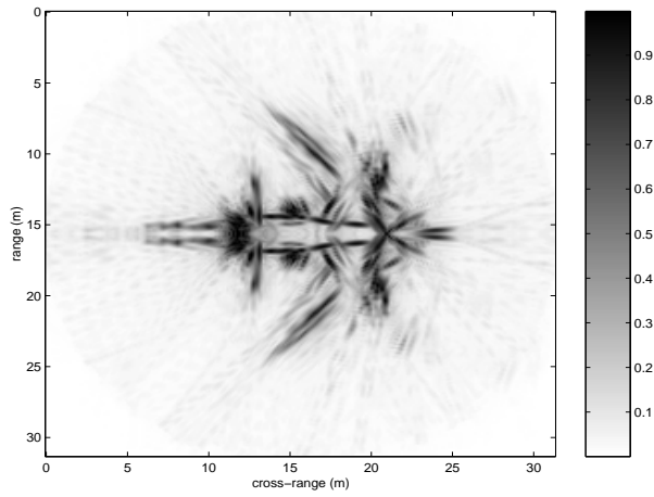
Fig. 8. Synthesized image by DFR from sub-aperture images, each sub-aperture width is 7 degrees.
