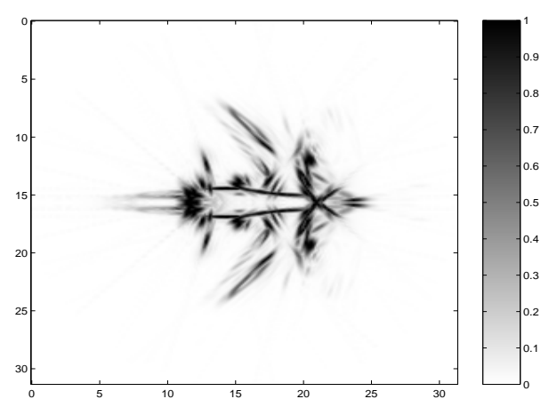
Fig. 10. Synthesized image by SPWVD from instantaneous images.
