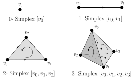
Fig. 1. Oriented simplices of dimension zero through three.
