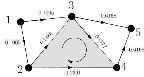
Fig. 3. A simplicial complex K of dimension 2. The numbers labelled on the edges correspond to the corresponding components of one of the two zero-eigenvectors of the 1-Laplacian of K .
