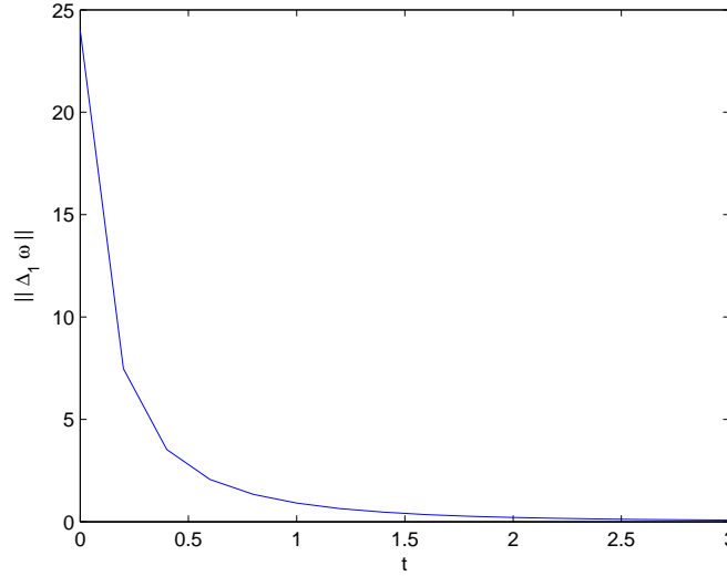
Fig. 7. The graph of \|\Delta_1\omega(t)\| against time shows an asymptotic convergence to zero.
