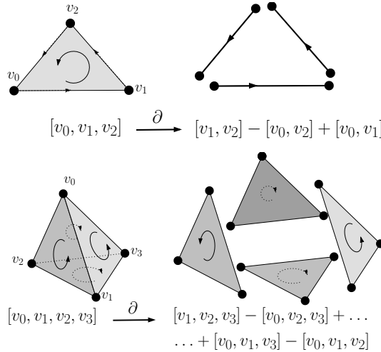
Fig. 2. The boundary operator on a 2-simplex [top] and a 3-simplex [bottom].
