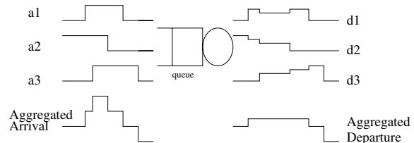
Fig. 14. Example of flow aggregation
