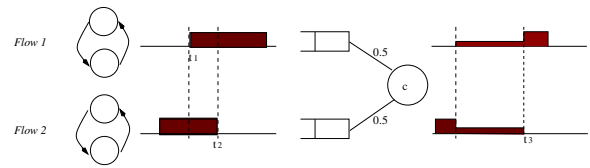
Fig. 16. A two queue weighted fair queueing system
