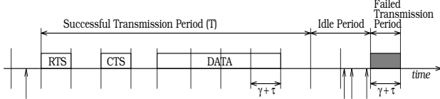
Fig. 10. Slotted MACA transmission periods
