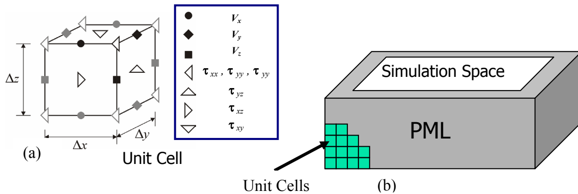
Figure 2: (a)The unit cell for the FDTD model. (b) The solution space for the FDTD simulation: composed of unit cells. The center is the area of the simulation while the edges are terminated by a perfectly matched layer (PML).
