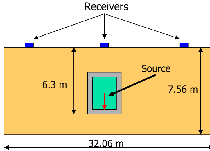
Figure 6: Layout of Case 1: Source located inside the structure
