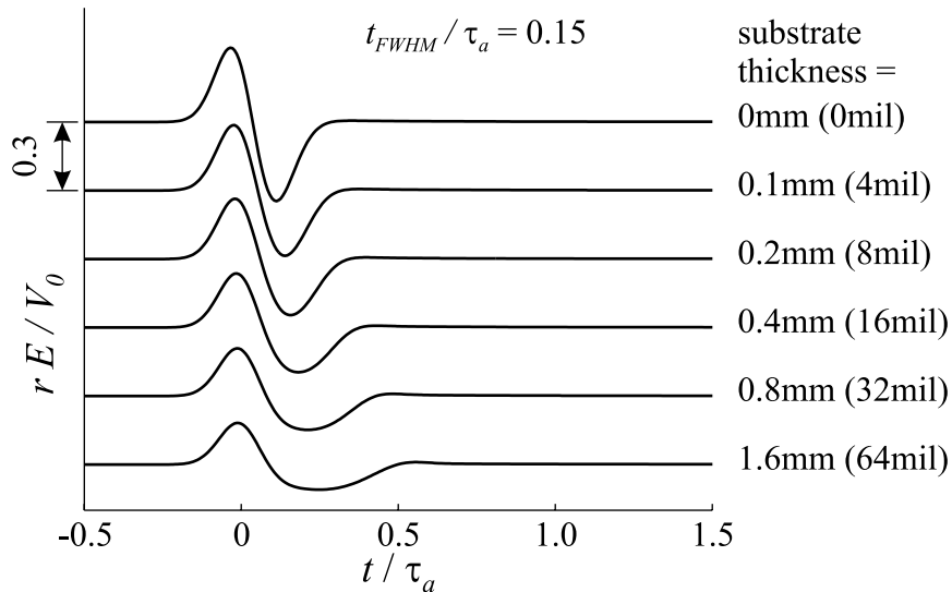
Figure 4. Normalized Radiated fields as functions of time for a Gaussian pulse with t_{FWHM}/\tau_a = 0.15 incident in a 100\Omega transmission line. Each line represents the radiated field on boresight of an RVD with 2\alpha = 60^\circ printed on an FR-4 substrate ( \epsilon_r = 4.2 ) whose thickness varies from 0 to 1.6mm.
