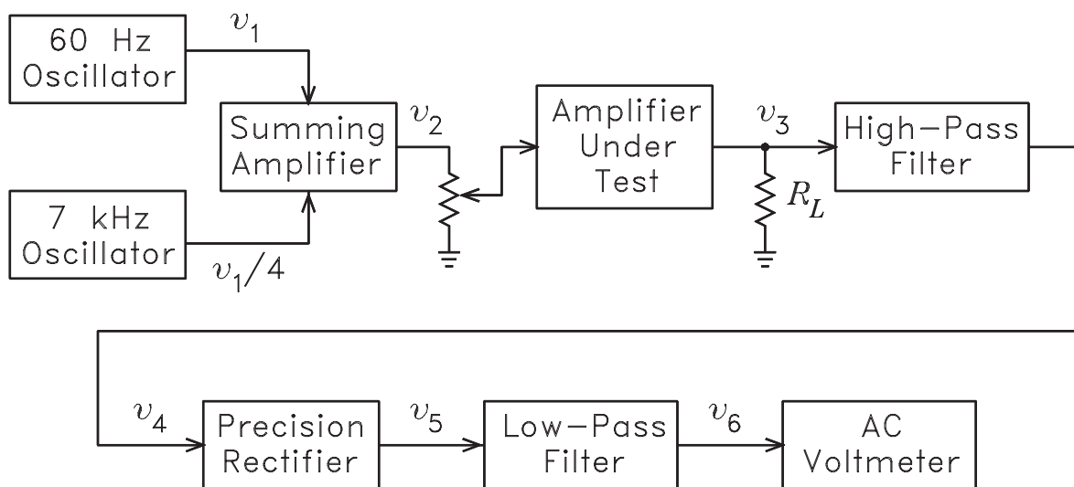
Block Diagram of IM Distortion Analyzer
