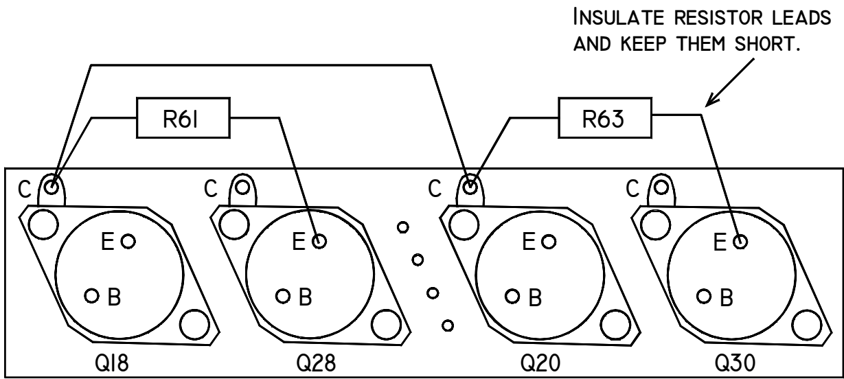
BOTTOM VIEW OF HEAT SINK CHANNEL
